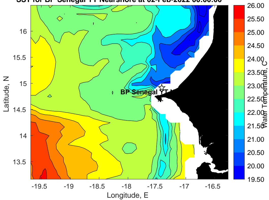
SST for BP Senegal YT Nearshore at 02-Feb-2022 00:00:00
